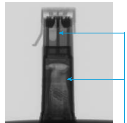
X-ray image showing air bubbles in printhead when using non-HP inks
