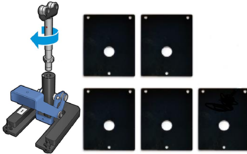
Figure 1: Shaft, support base and shims
